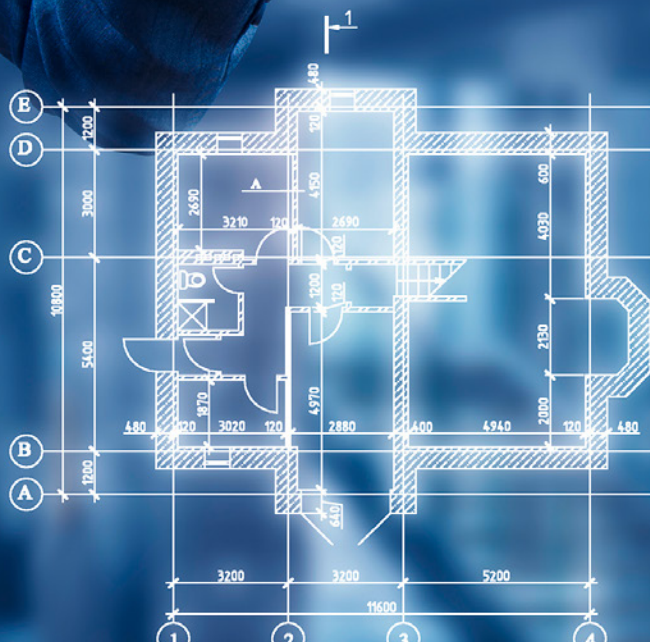
basement Plan
