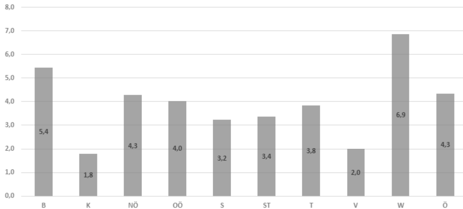
ICU Belag Covid-19 / 100.000 Ew BL 2021_05_10
